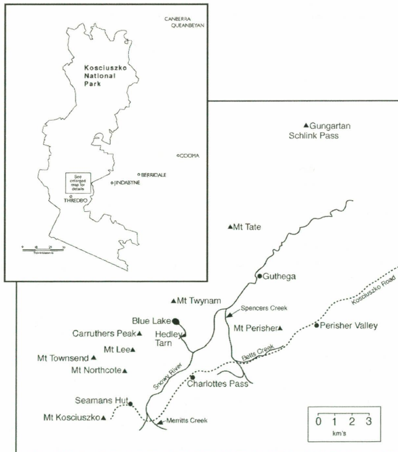
Figure 1: General location of the threatened alpine plants and place names referred to in this recovery Plan
