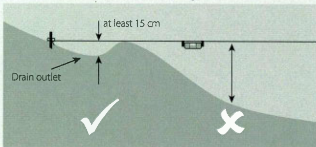
Figure 5.13: Measuring effective bank height
