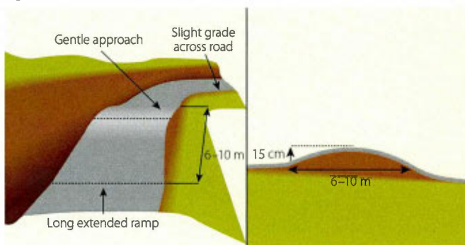
Figure 5.11: Rollover bank
