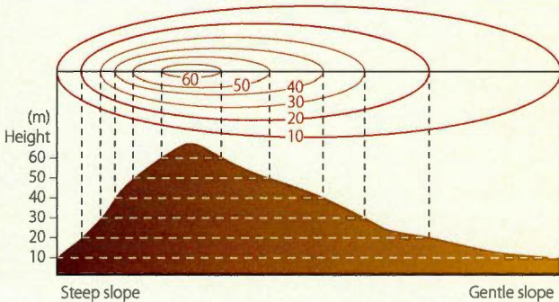
Figure 7.3: The relationship between contour lines and slope
