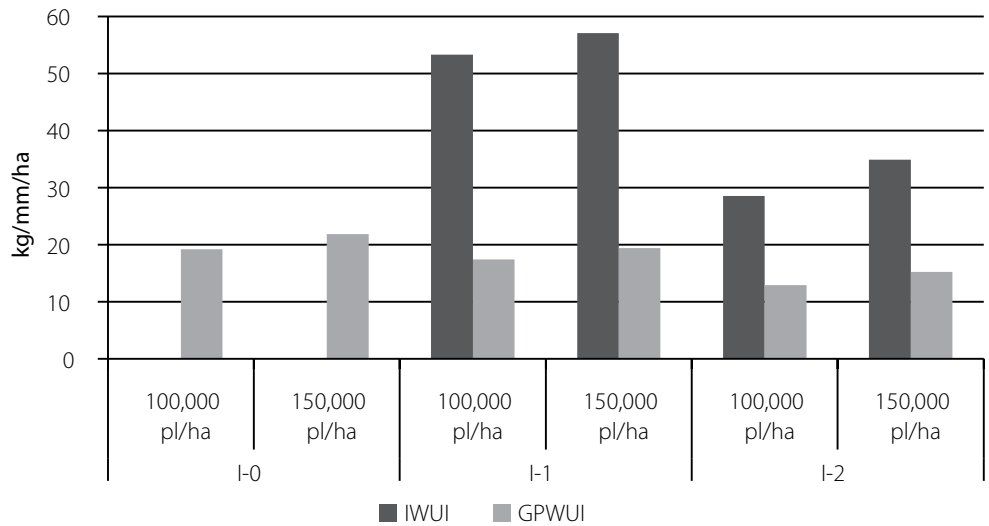
Figure 4. Experiment IWUI (yield/applied mm) and GPWUI (yield/total in-crop mm)
